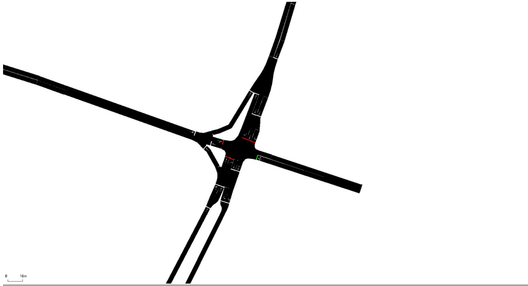
Figure 3.1: Custom SUMO intersection used for dataset generation and DRL training.
