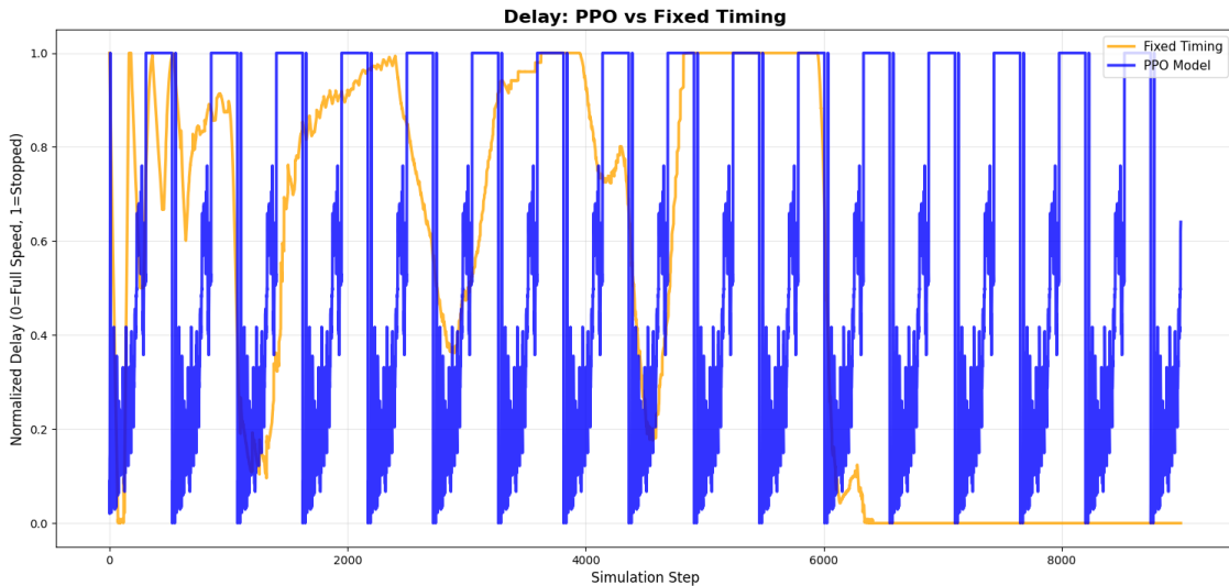
Figure 4.4: Average delay comparison between fixed-time and PPO controller.
