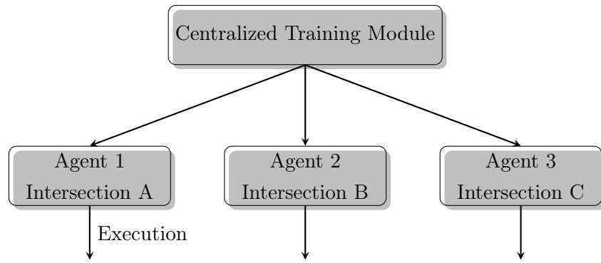
Figure 2.8: Centralized training and decentralized execution in Multi-Agent RL.
