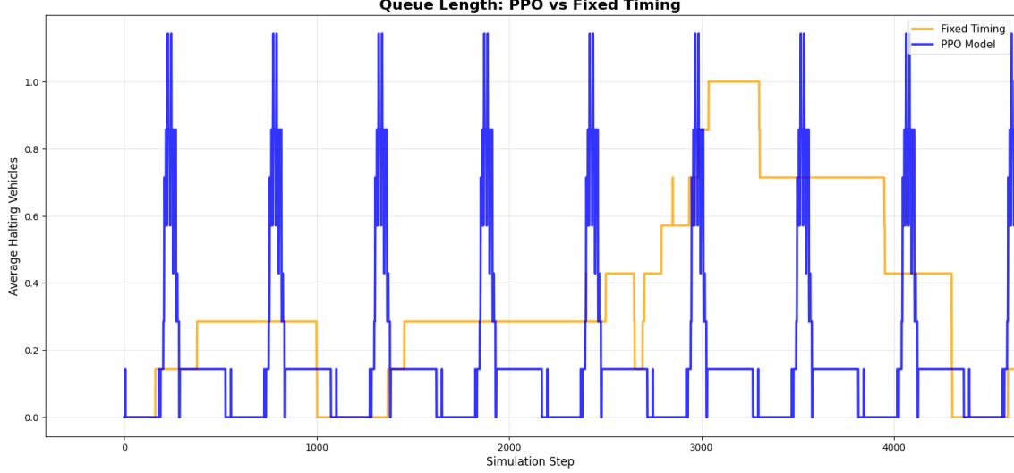
Figure 4.5: Average queue length comparison between fixed-time and PPO controller.
