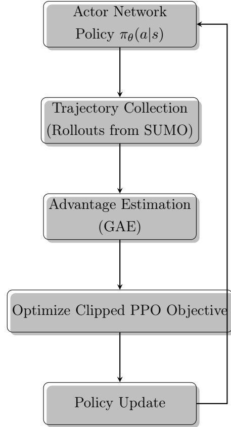
Figure 2.7: Proximal Policy Optimization (PPO) workflow.
