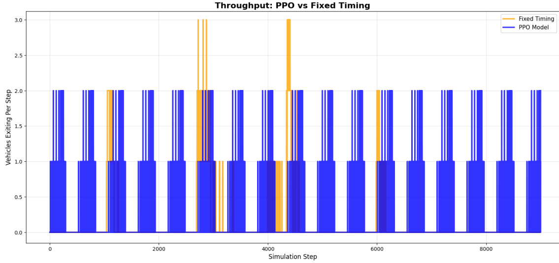
Figure 4.6: Vehicle throughput comparison between fixed-time and PPO controller.
