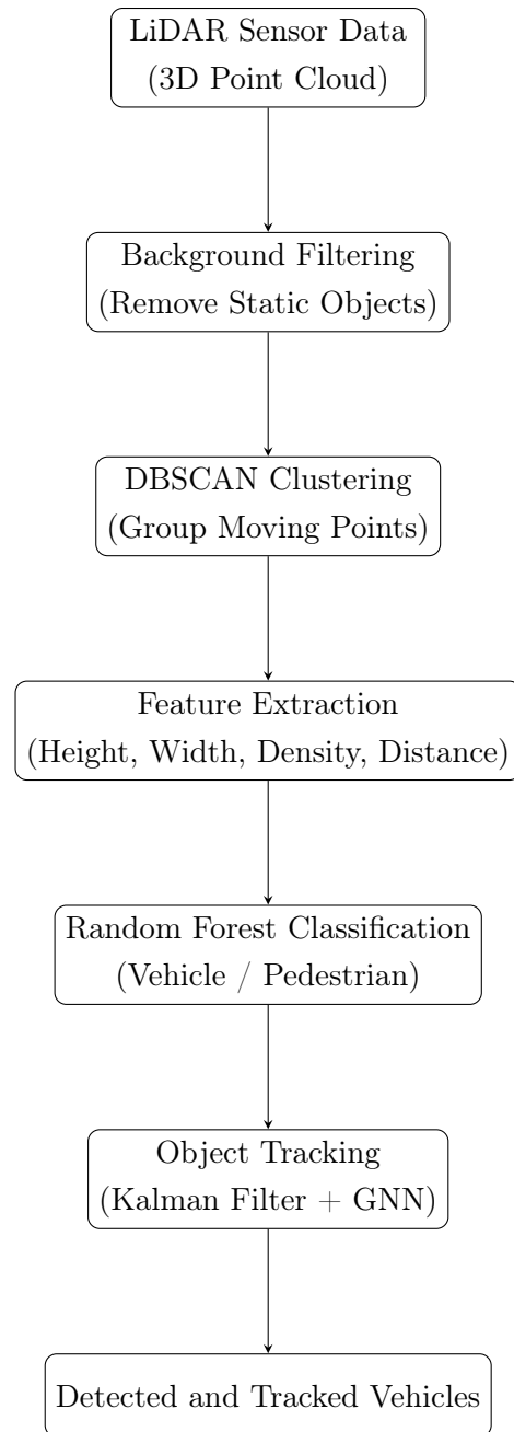
Figure 2.3: Block diagram of the LiDAR-based vehicle detection system.
