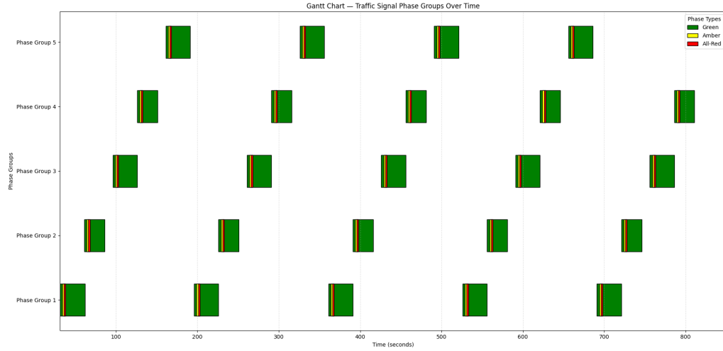
Figure 4.2: SUMO gantt chart showing phase durations with the fixed-time traffic signal controller.
