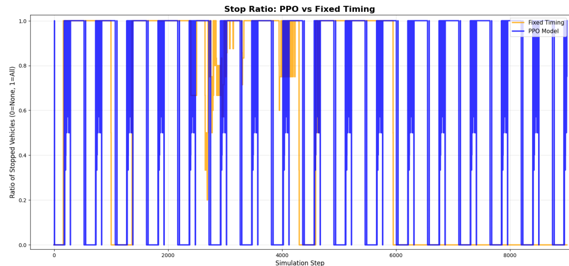
Figure 4.7: Stop ratio comparison between fixed-time and PPO controller.
